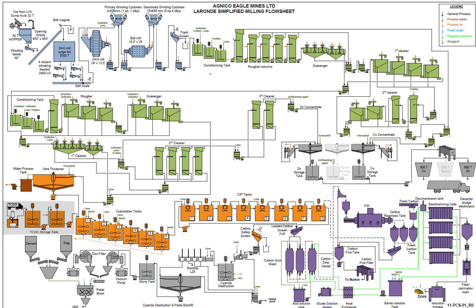
Flowsheet for LaRonde mill (7,200 tpd milling rate)
