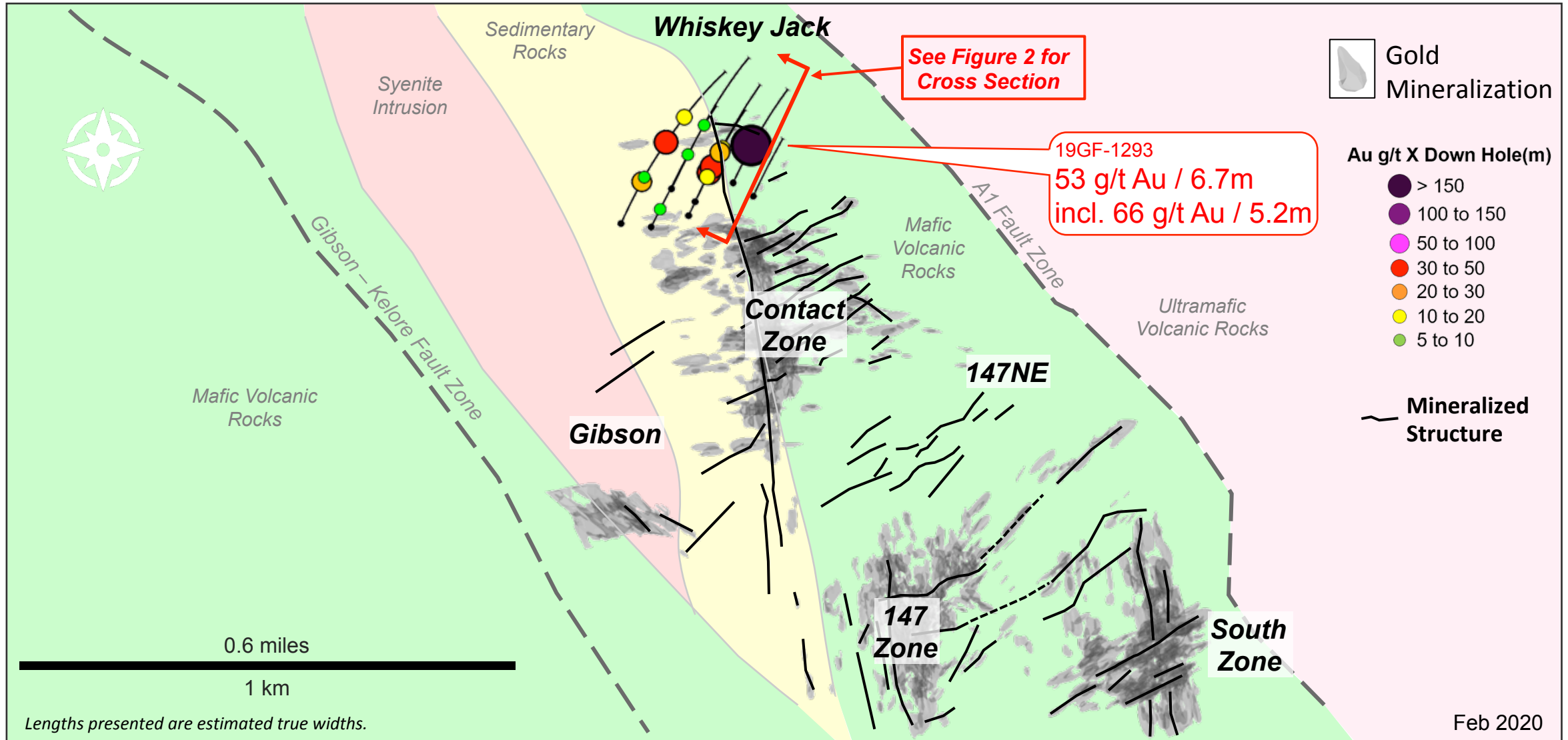
Figure 1: Grey Fox Area Mineralization & Whiskey Jack Drill Hole Locations - Plan View
