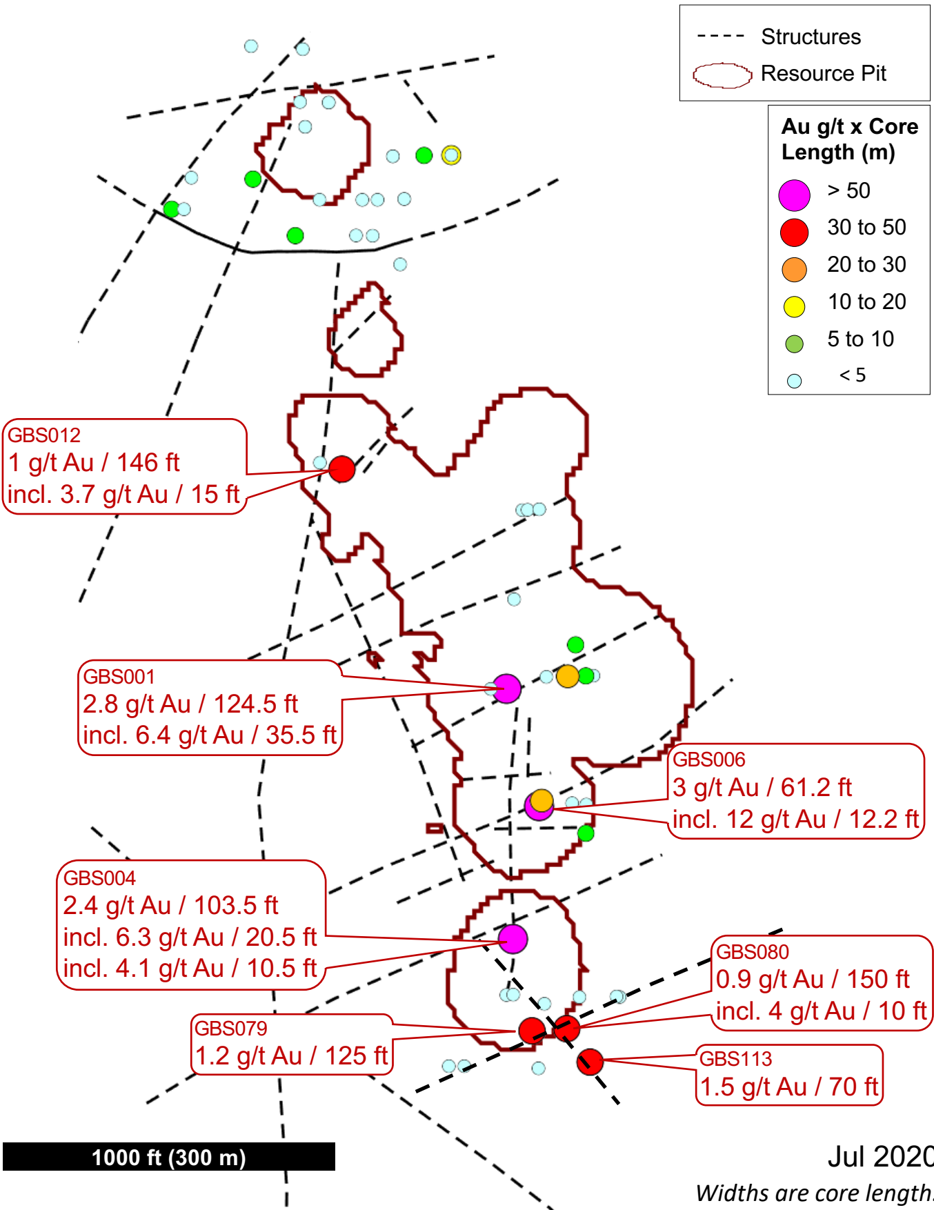
Figure 2: Gold Bar South – Plan View
