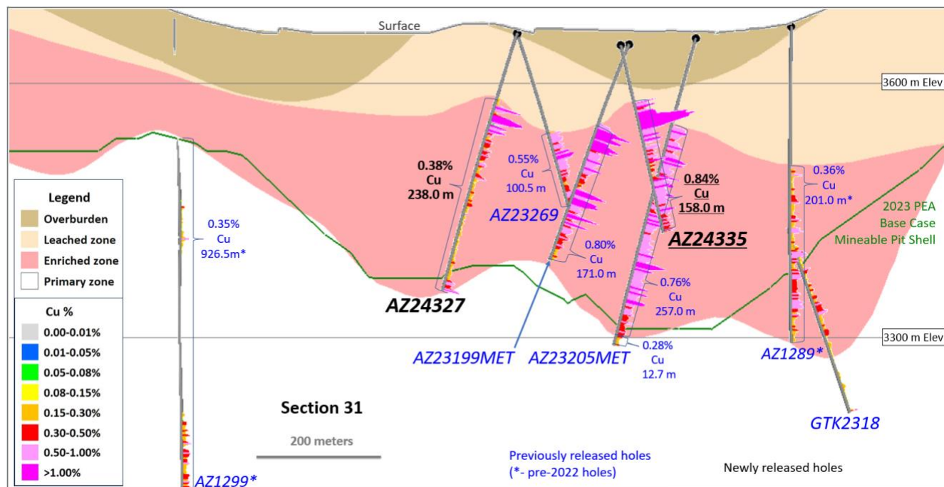
Figure 6 - Section 31 - Drilling, Mineralized Zones and 30-Year PEA Pitshell (Looking Northwest)
