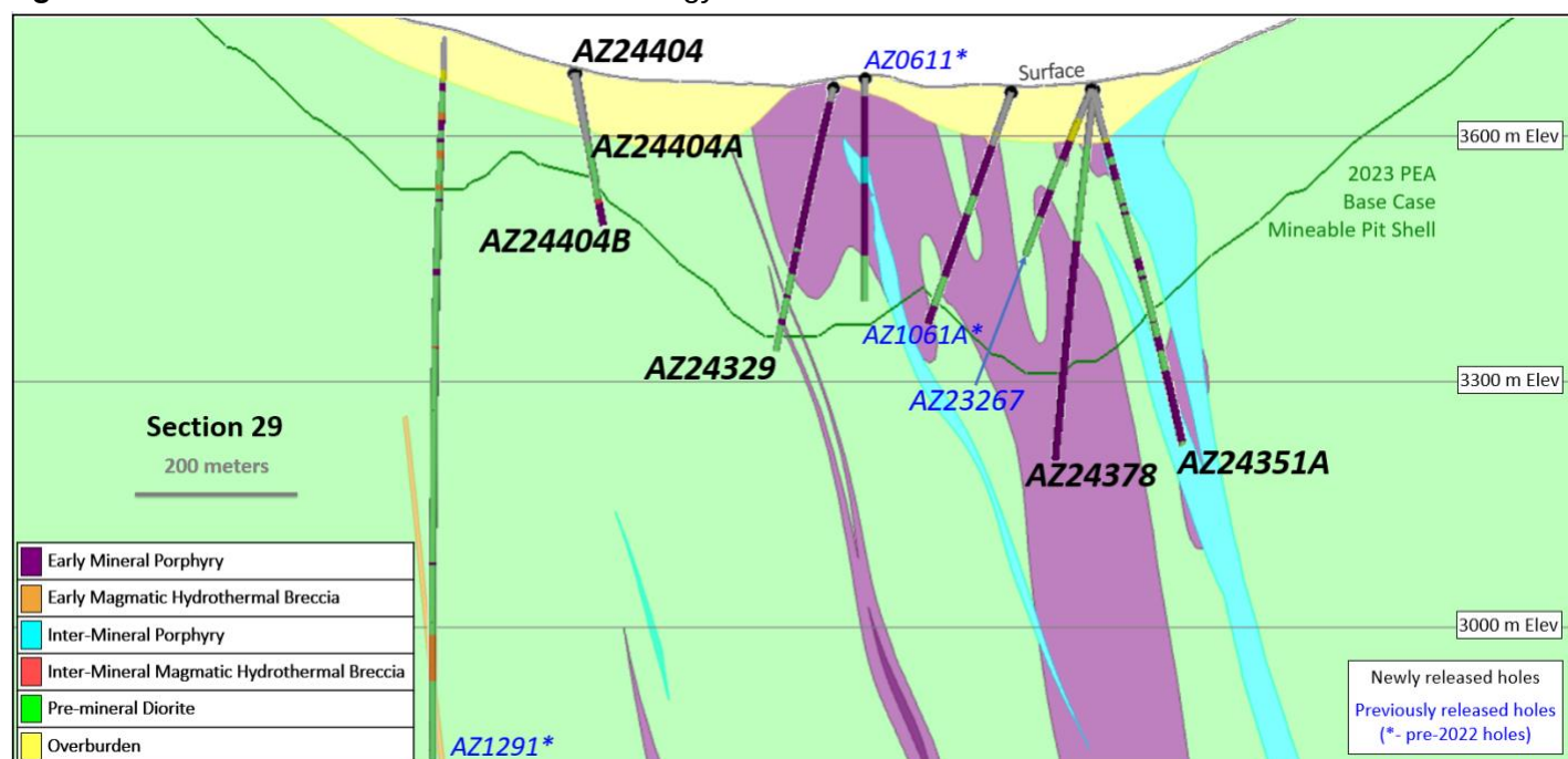
Figure 8 - Recent Drill Data and Inferred Geology in Cross Section 29
