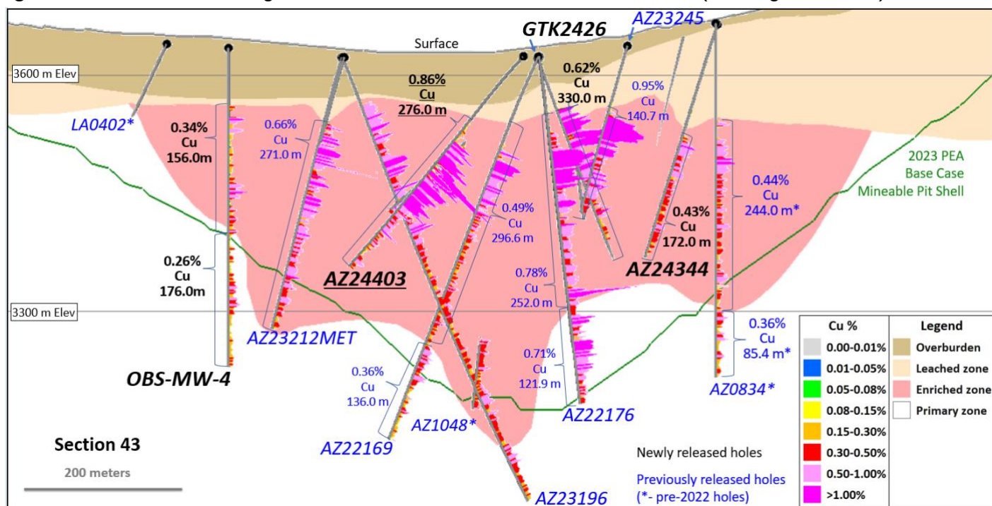
Figure 4 - Section 43 - Drilling, Mineralized Zones and 30-Year PEA Pitshell (Looking Northwest)
