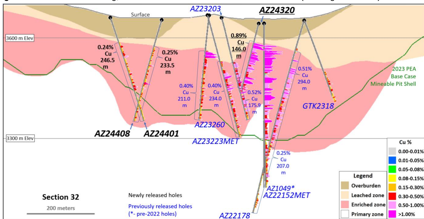
Figure 5 - Section 32 - Drilling, Mineralized Zones and 30-Year PEA Pitshell (Looking Northwest)
