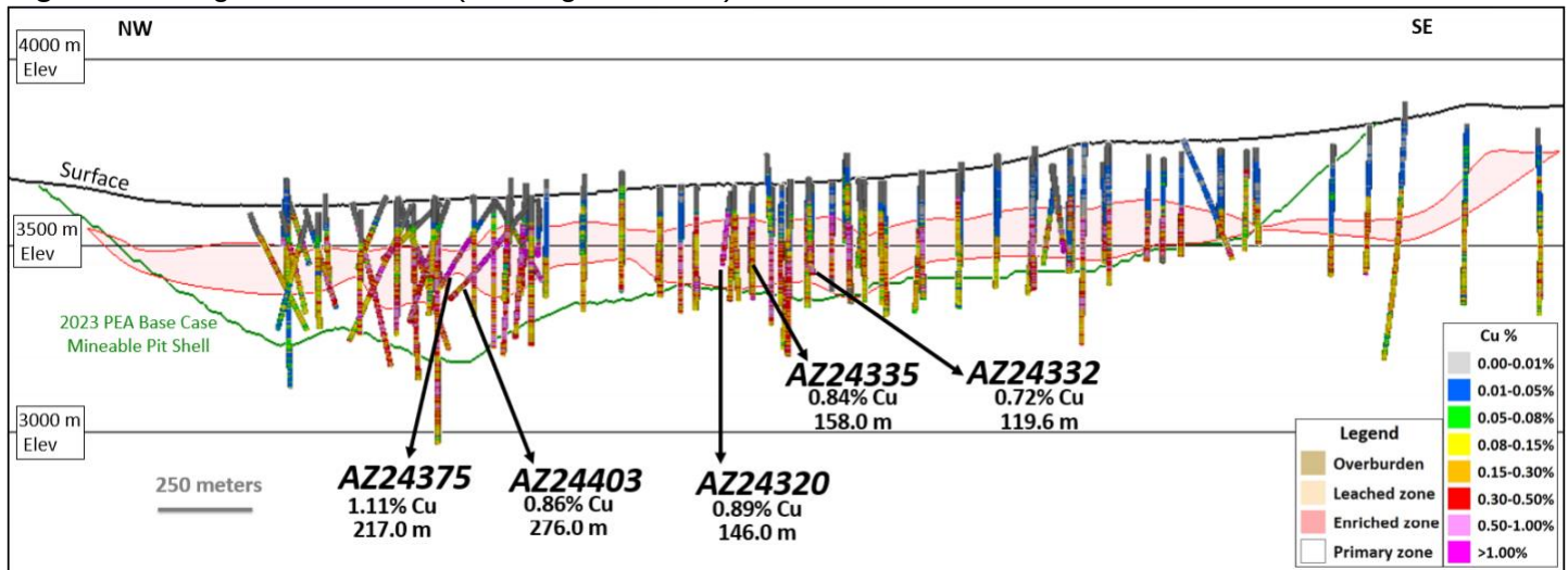
Figure 2 - Longitudinal Section (Looking Northeast)
