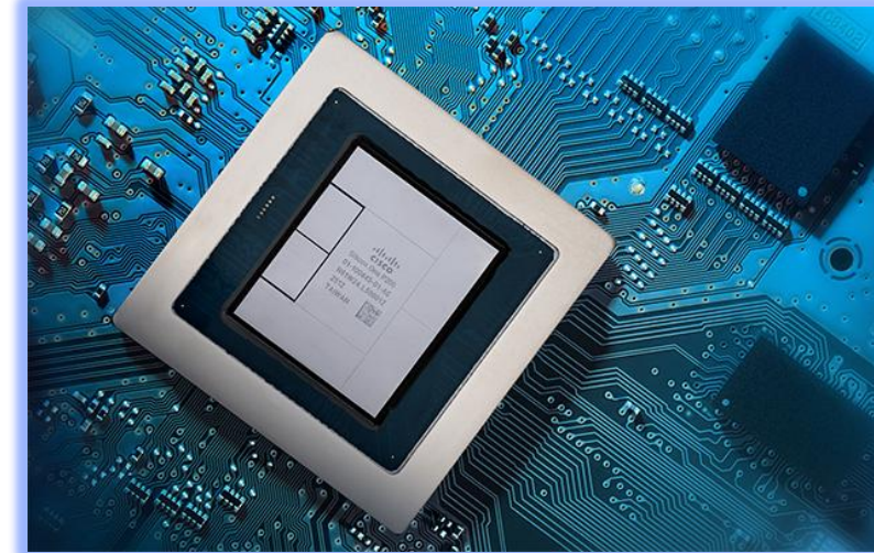
Cisco Silicon One P200
