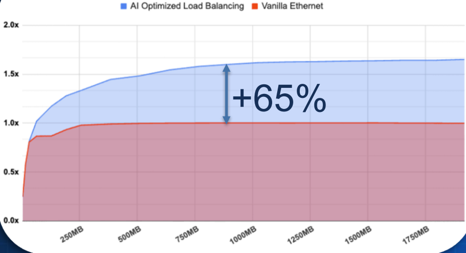
NCCL All-to-All Performance
