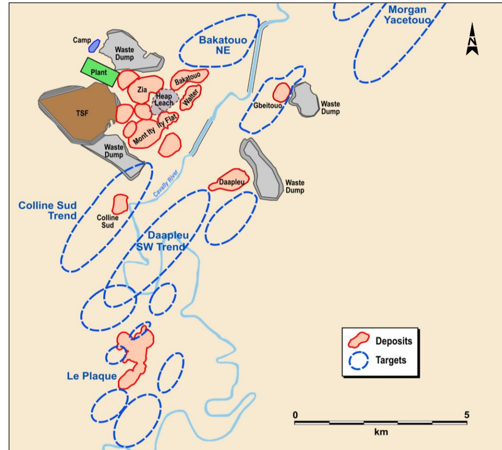
Simplified Ity Site Map and Exploration Targets
