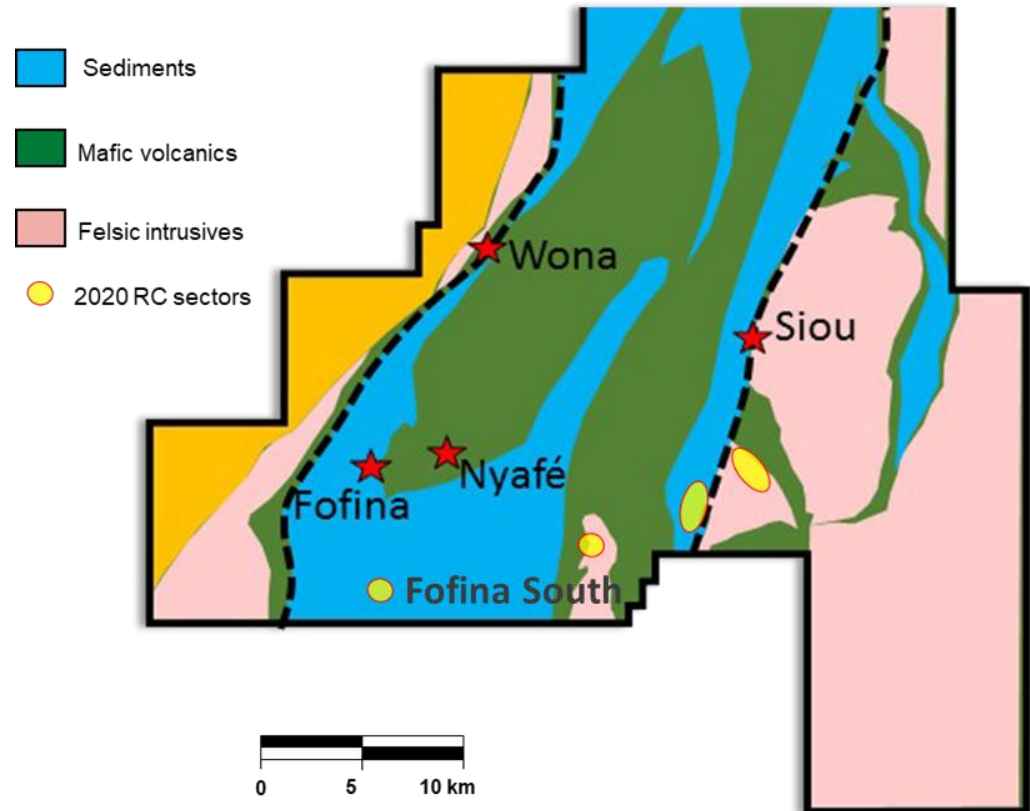
Mana exploration map
