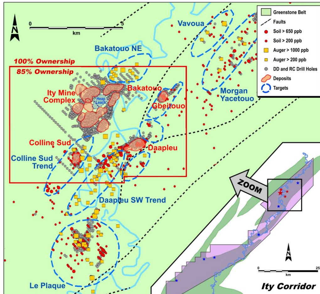
Ity mine drilling targets
