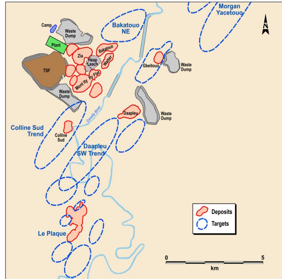
Simplified Ity map with exploration targets
